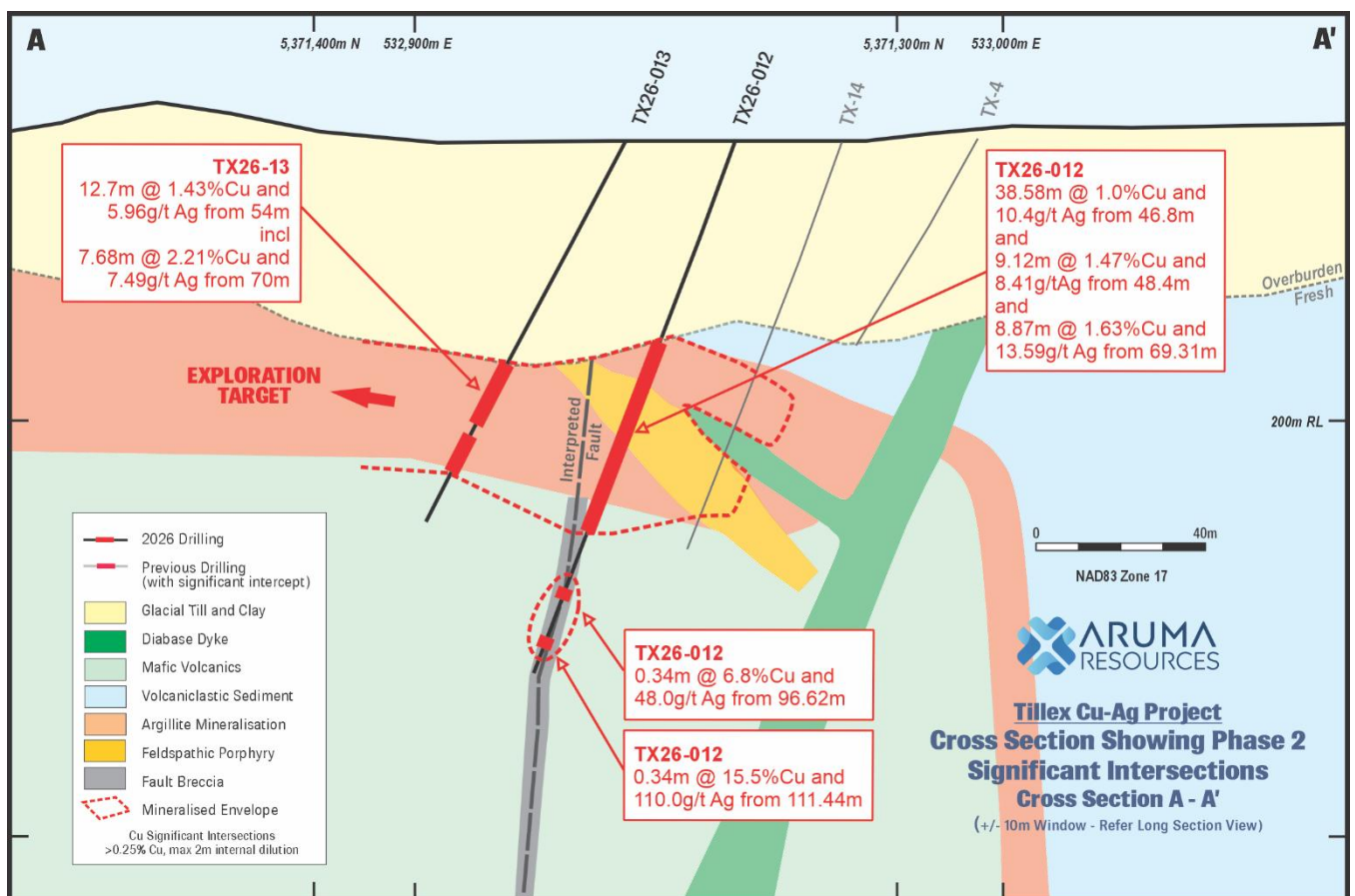
Figure 2: Tillex Geological Cross Section Cross Section A-A' showing drillholes TX26-012 and TX26-013 (Refer Figure 1).
