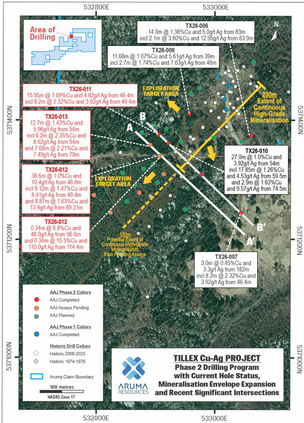
Figure 1: Tillex Project – Intersections from Phase 2 drilling completed to date, with results reported in this announcement in red and previous Phase-2 results in black. Also showing, pending and planned Phase-2 holes, plus Aruma Phase-1 drilling and historic drilling.
