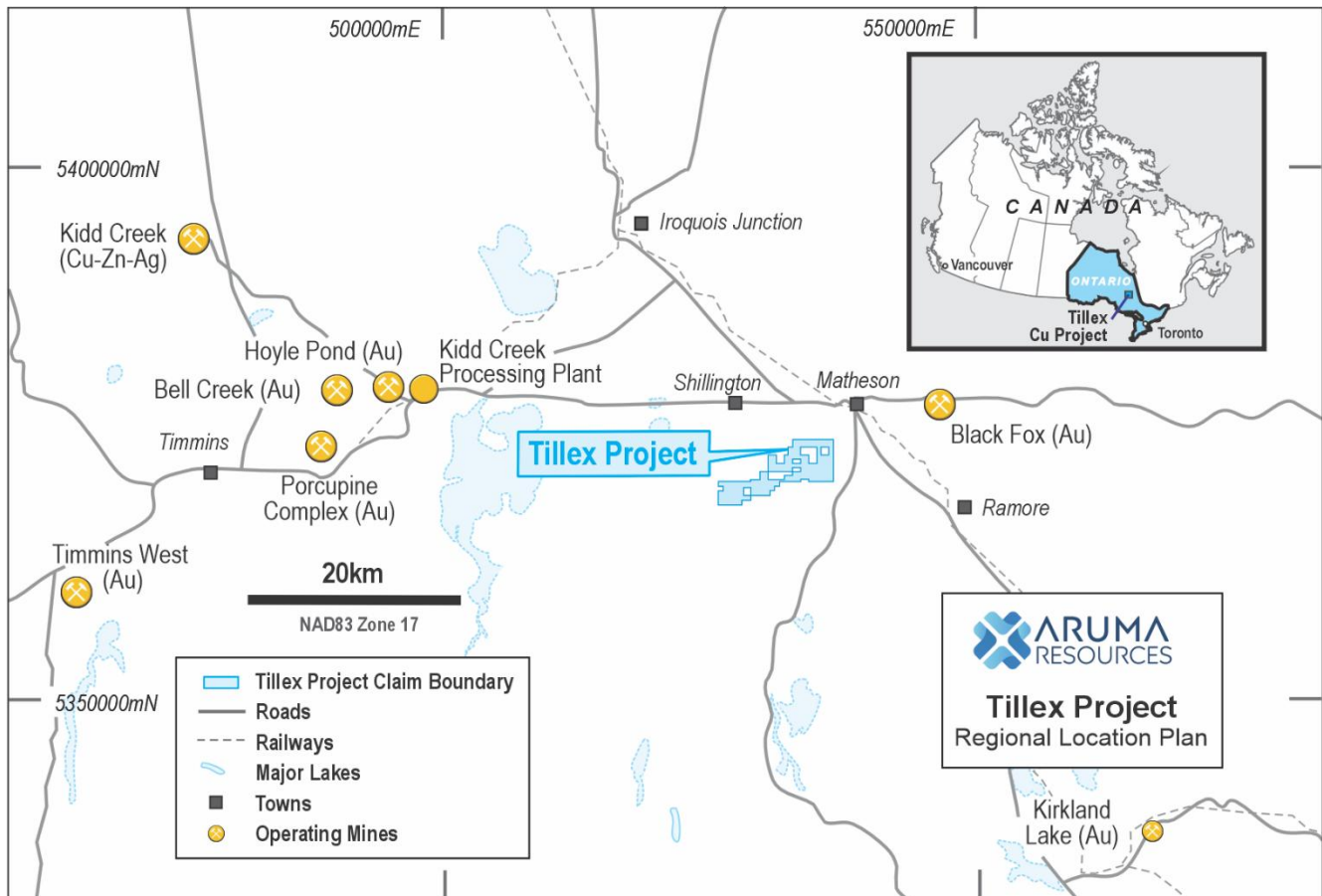
Figure 2: Regional location map showing Tillex Project within the Timmins mining district, Ontario, Canada
