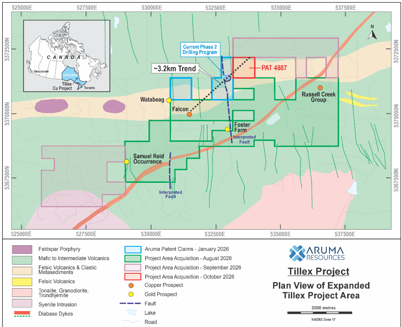
Figure 1: Expanded Tillex Project area, showing the newly acquired patented mineral right PAT4887, and the extended interpreted 3.2km Tillex Trend.
